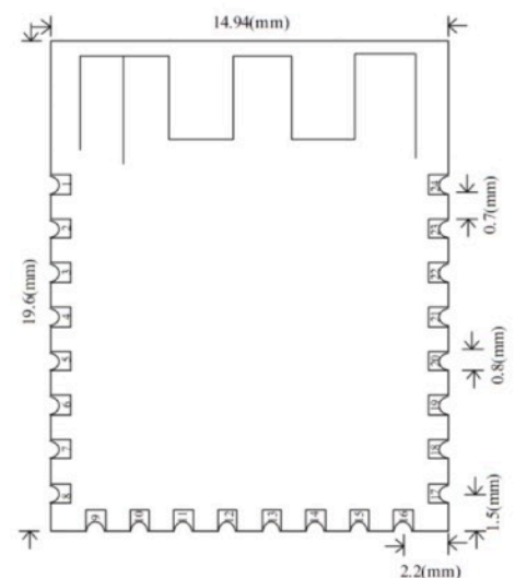
Dimension (mm)
